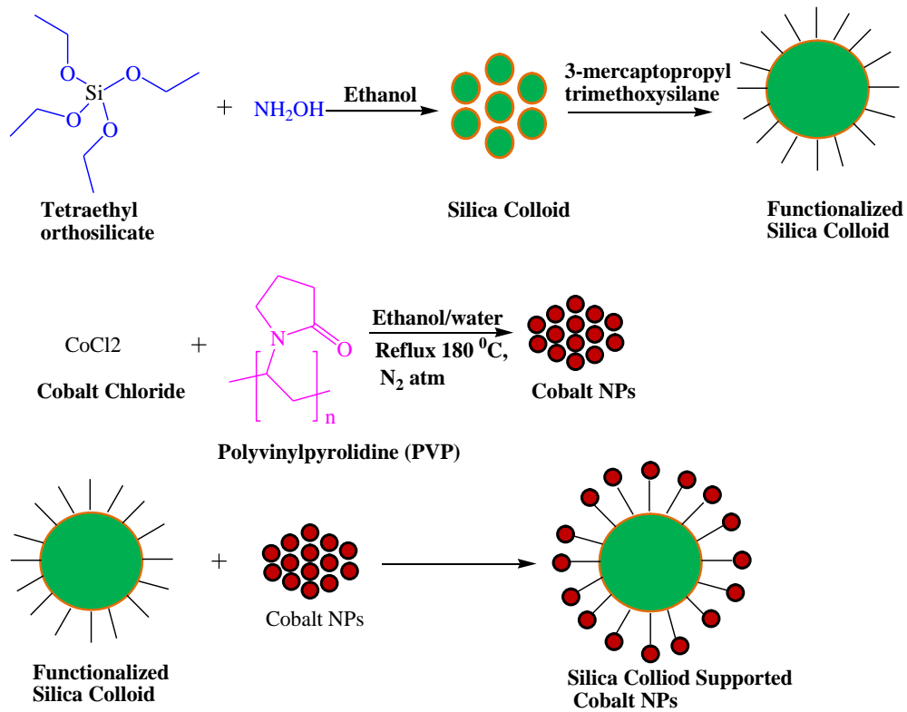
Scheme 1: Schematic representation of synthesis of colloidal silica supported Co NPs.
