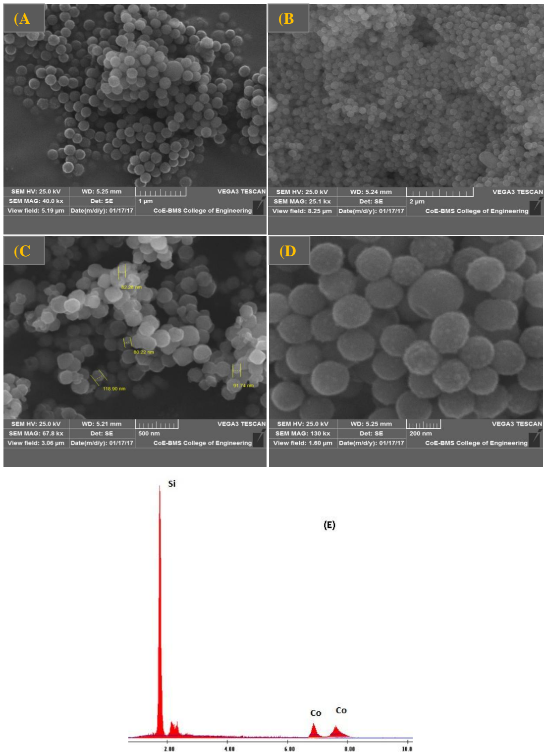
Figure 2:(a) SEM images of (A) Si Colloid, (B) Thiol capped Si Colloid and (C) Co NPs, (D) Silica supported Co NPs and (E) EDX pattern of silica supported Co NPs.
