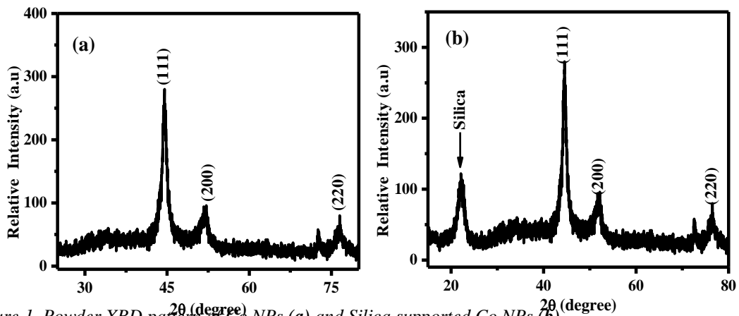
Figure 1. Powder XRD pattern of Co NPs (a) and Silica supported Co NPs (b).
